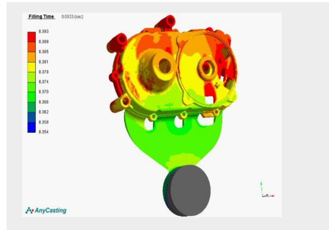
Filling Time, Material Flow
